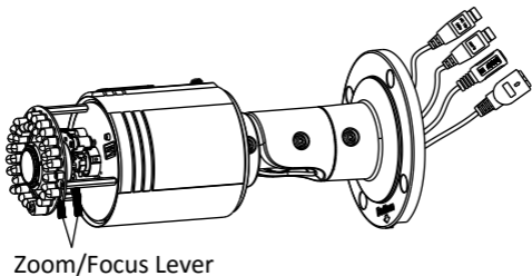
Figure 2-9 Zoom and Focus Adjustment
