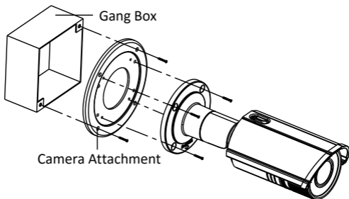
Figure 2-7 Secure the Camera
