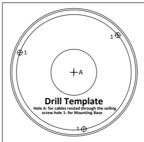
Figure 2-1 Drilling Template
