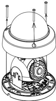
Figure 2-8 Disassemble the Camera
