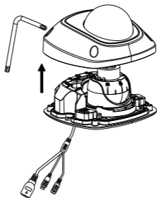
Figure 2-3 Disassemble the Camera
